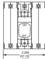
Three Pole
