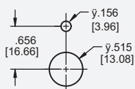
Single Pole
