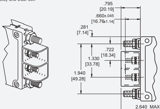
Relay and Dual Coil
