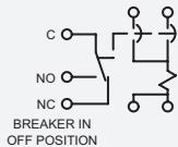
Series Parallel with optional 1REC4 Auxiliary switch
