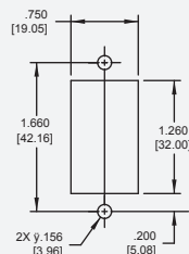
Panel Mounting Detail
