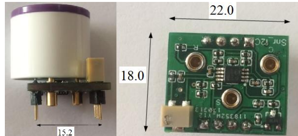
Figure 3 – Module Dimensions (units in mm)
